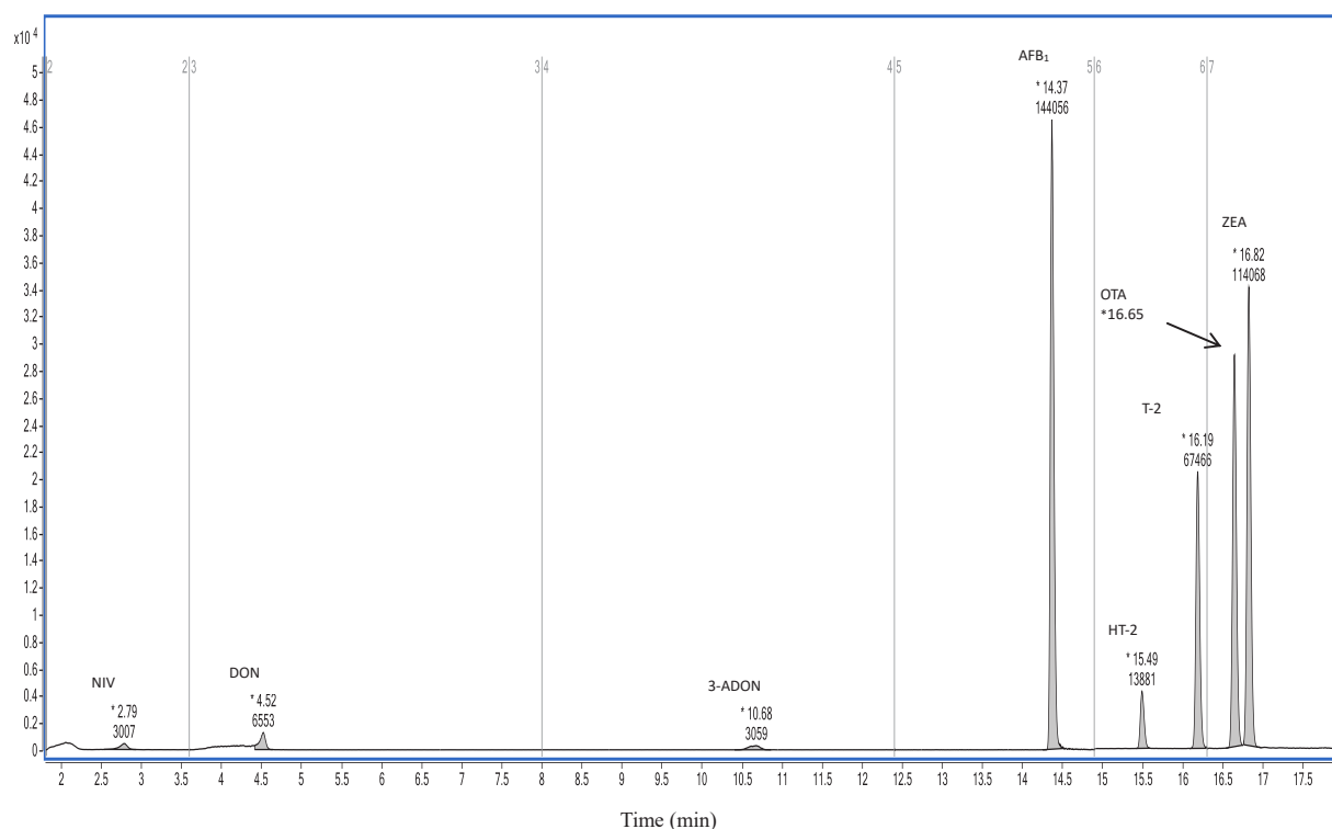
Figure 1. The chromatogram of nivalenol, deoxynivalenol, 3-acetyl-deoxynivalneol, aflatoxin B 1 , HT-2 toxin, T-2 toxin, ochratoxin A, and zearalenone at 100 ng/mL.
