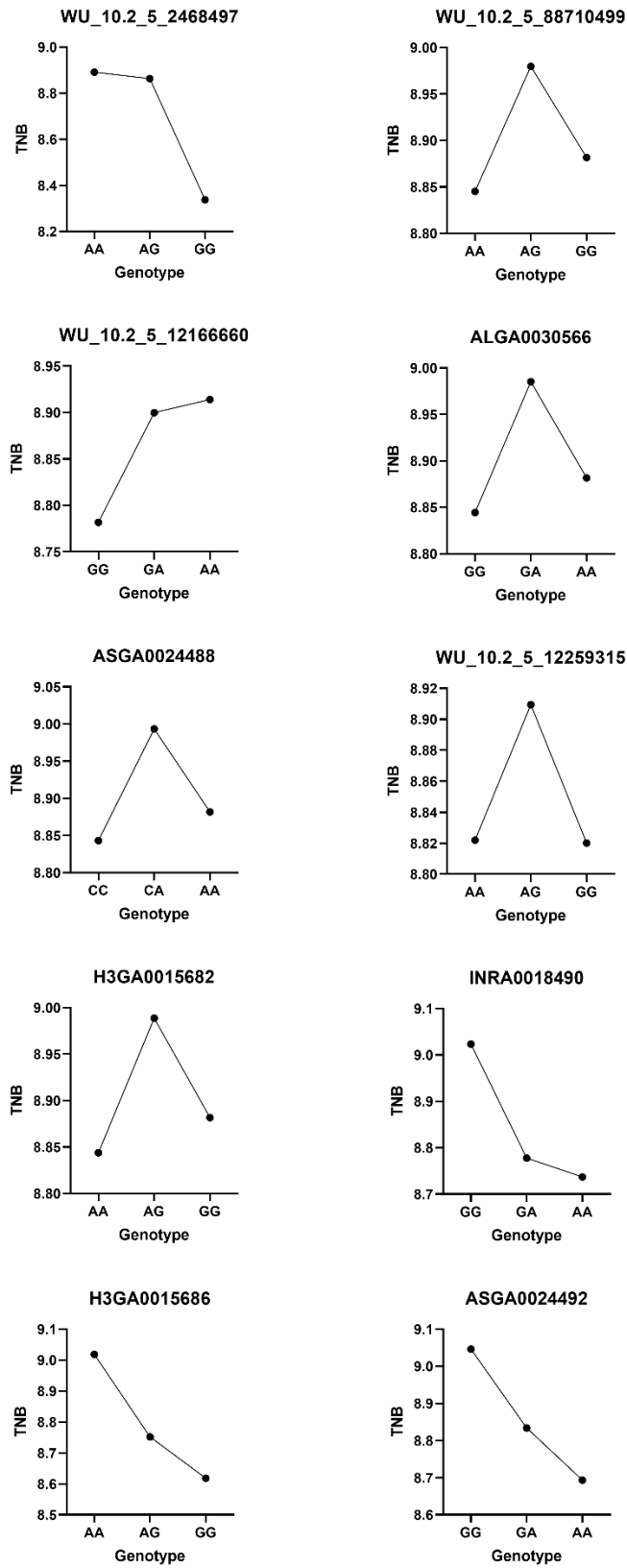
Fig S1. The phenotypic change according to the genotype of the markers that showed the highest genetic variance explained in TNB
