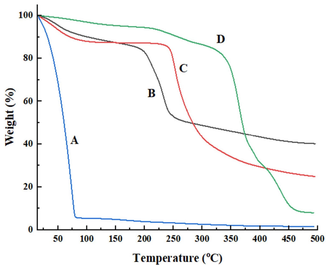
Figure S1. The thermogravimetric analysis (TGA) thermograms of (A) LPMB001, (B) AL, (C) AG and (D) LPMB001/AG-AL.
