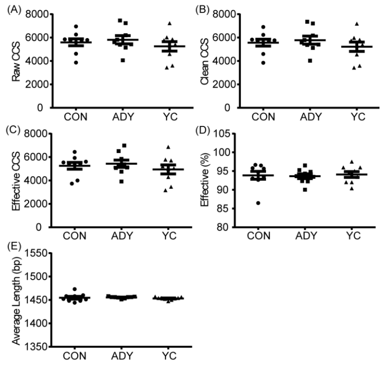
Figure S1. Summary of sequence statistics of all samples. (A) Raw CCS, (B) Clean CCS, (C) Effective CCS, (D) Effective, (E) Average Length. CCS, circular consensus sequences. CON, control group (n = 9); ADY, active dry yeast group (n = 9); YC, yeast culture group (n = 9).
