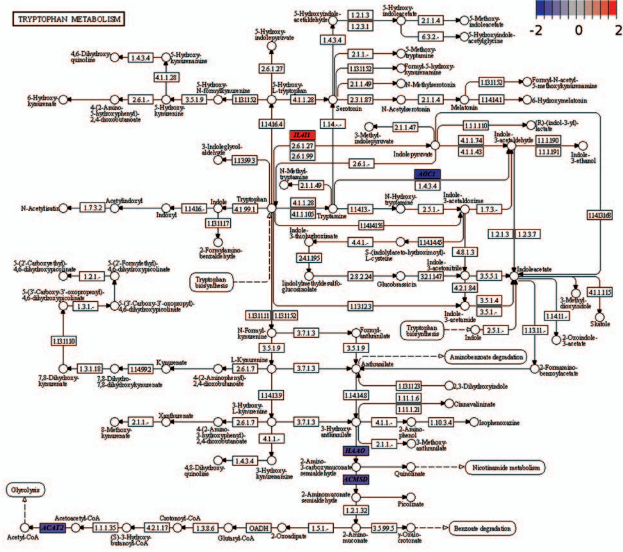
Data on KEGG graph Rendered by Pathview
